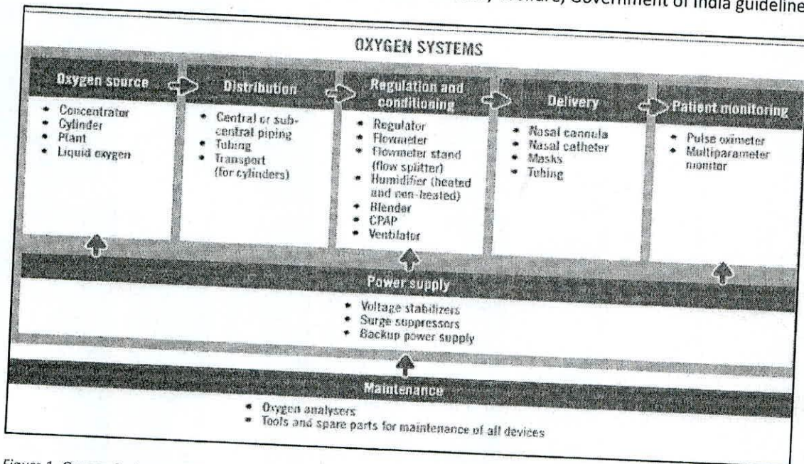
Figure 1- Oxygen System components (Source WHO)
